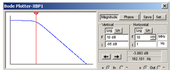
P1b (Circuit frequency response)
