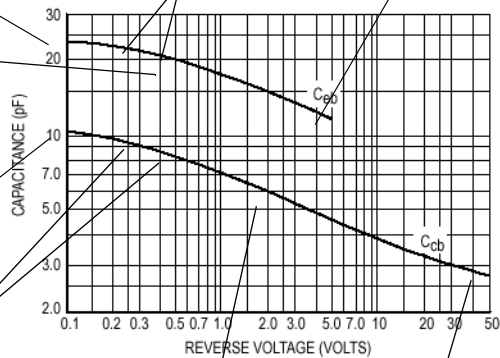
Figure 9. Capacitances
