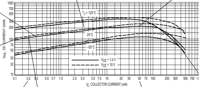
Figure 3. DC Current Gain
