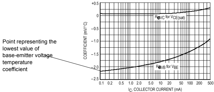
Figure 12. Temperature Coefficients
